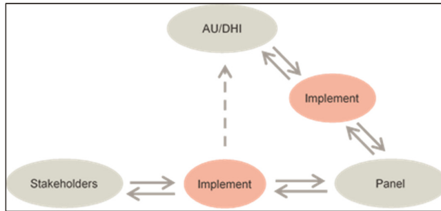
Figure 1. Communication model
